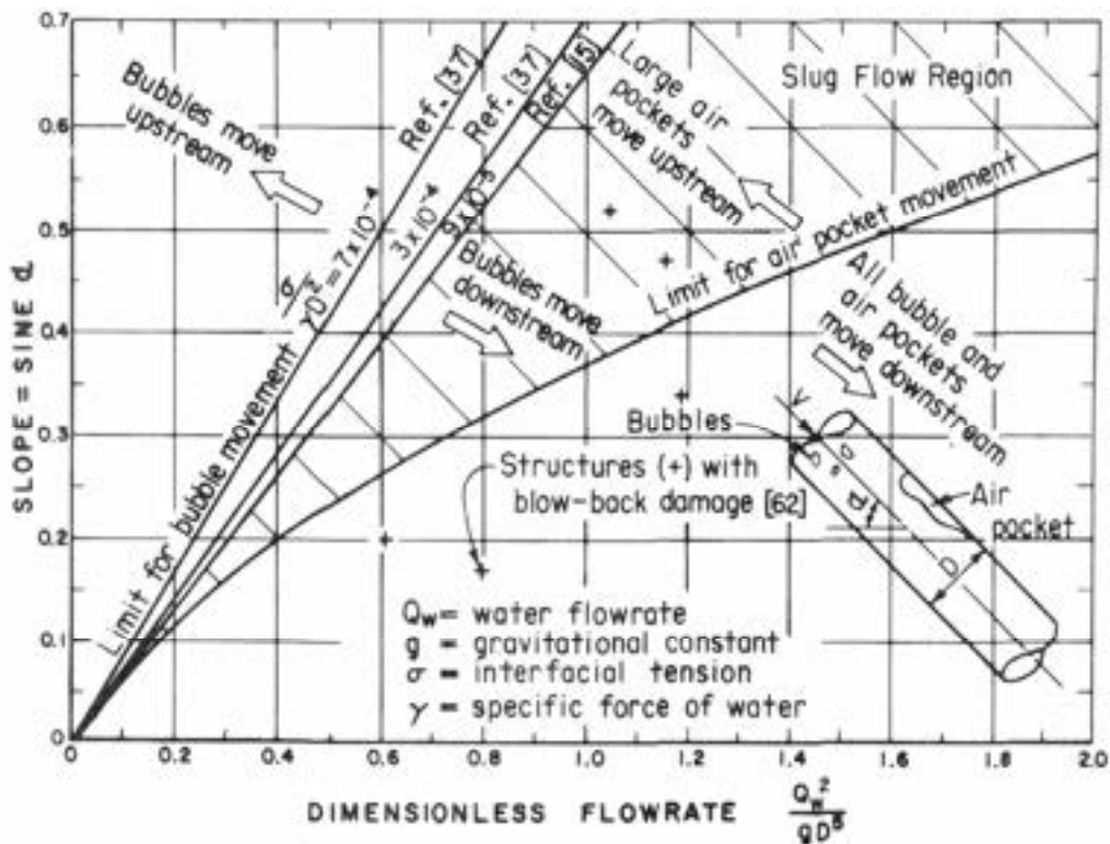
Figure 12 Graph showing flow rates required to transport air bubbles and pockets in pipes of varying slope (taken from Falvey, 1980)
