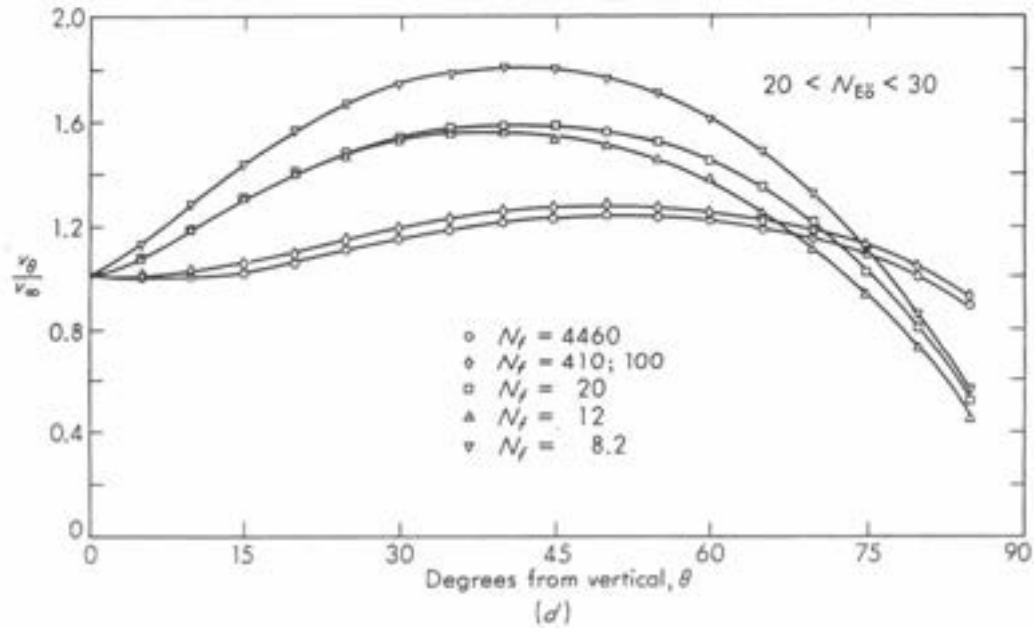
Figure 9d Rise velocity of slug-flow bubbles in inclined pipes for 20 < N_{E0} < 30 (taken from Wallis, 1969)
