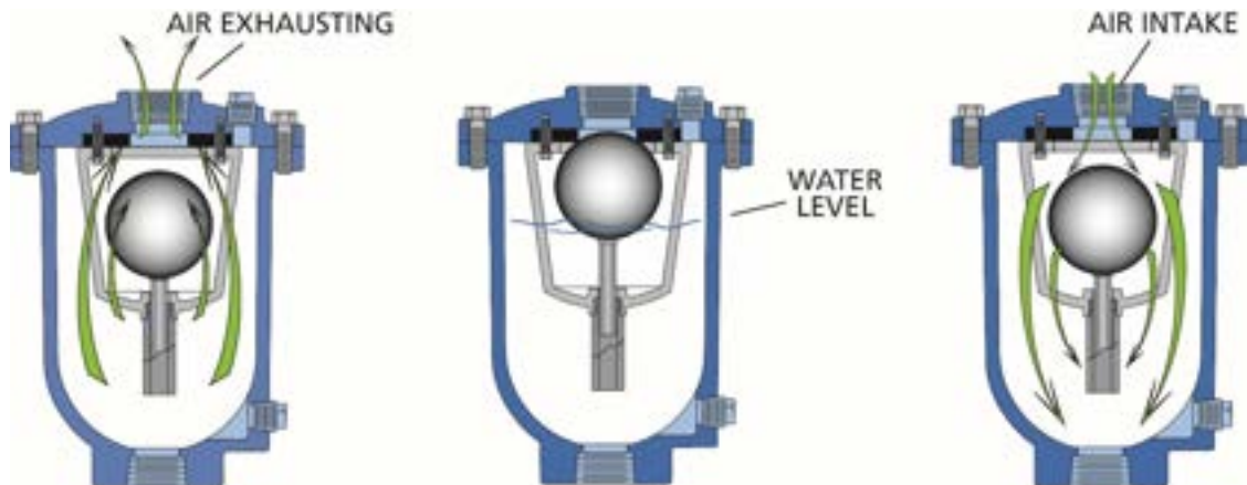
FIGURE 9. Air/Vacuum Valves
