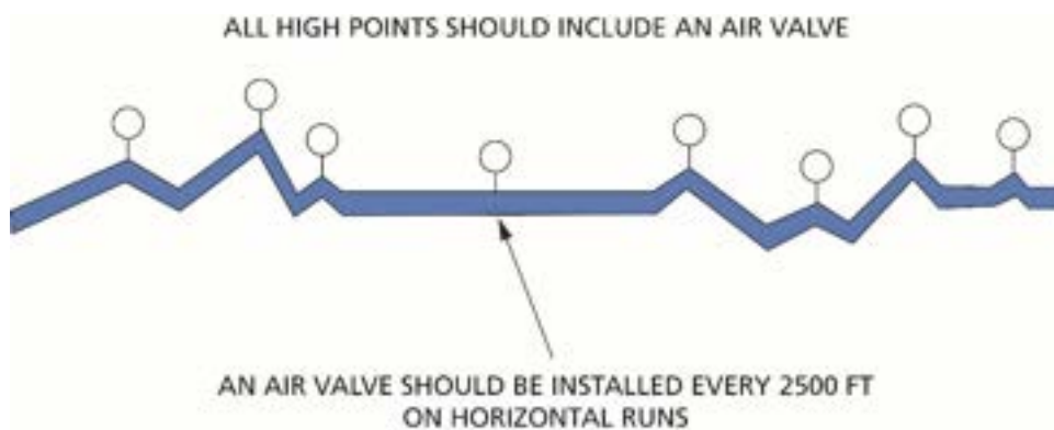
FIGURE 8. Air Valve Placement
